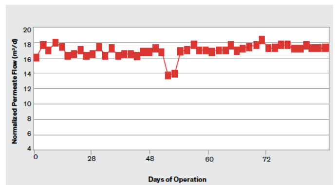
Figure 3: Normalized permeate flow registered at Rothera plant.
